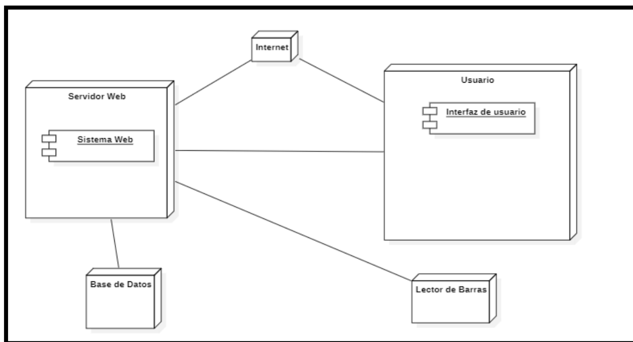
Diagrama 24: Despliegue
